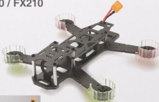
Carbon Fibre Frame with Lower Battery Position
